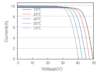
Current-Voltage Curve JAP72S01-325/SC/1000V
