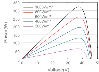
Power-Voltage Curve JAP72S01-325/SC/1000V
