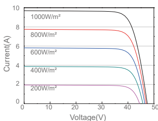
Current-Voltage Curve JAP72S01-325/SC/1000V
